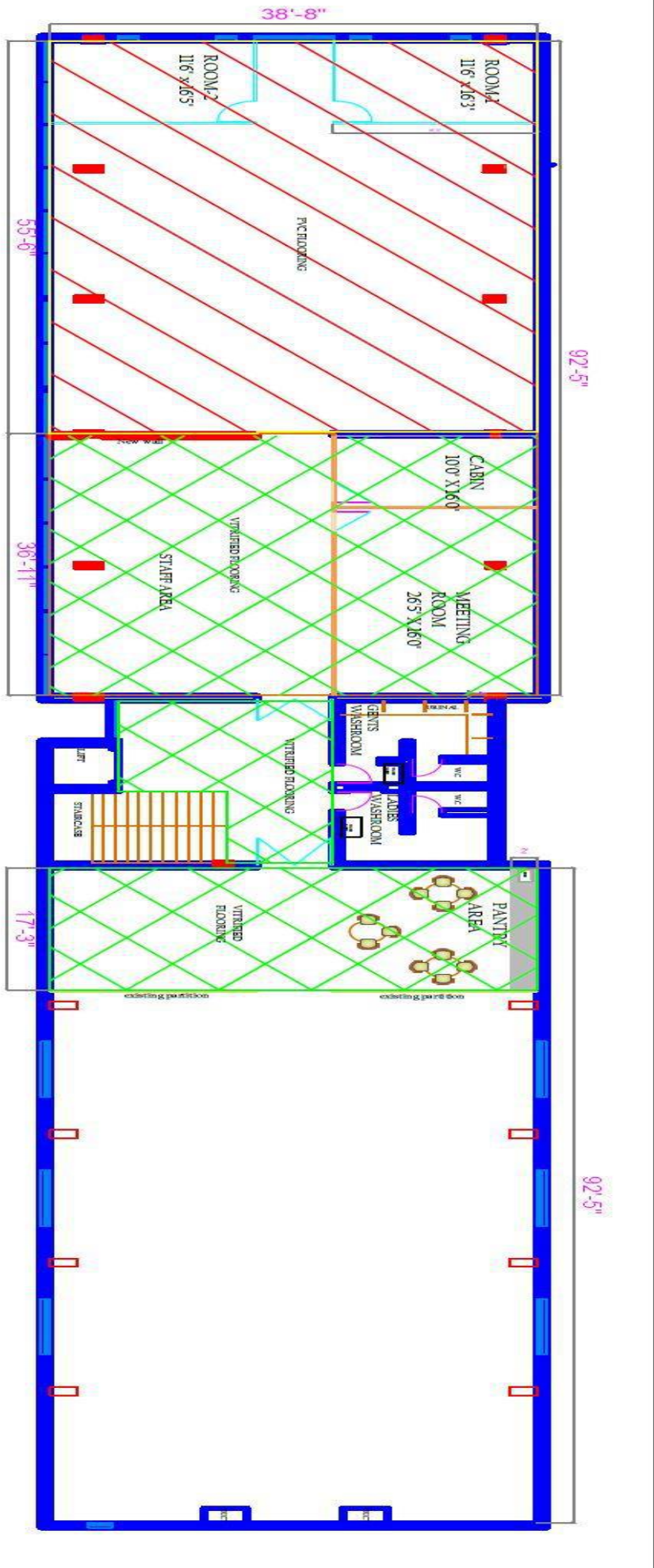
IRC BUILDING-4TH FLOOR PLAN
